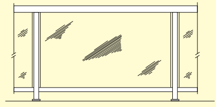
NS 6 - GLASS Single Toprail
